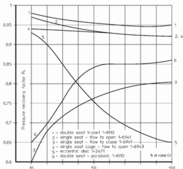
Figure 6 – Typical F_L values versus C_v % and flow direction for different PSM valve types.
